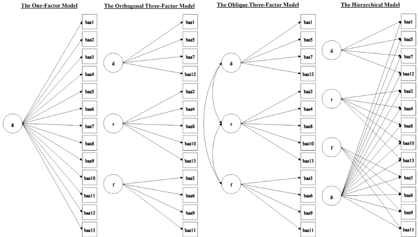
Fig. 1. Schematic diagrams of the four models tested in the current study. The models depicted from left to right are: (1) a one factor model, (2) an orthogonal three group factor model, (3) an oblique three group factor model, (4) a four-factor hierarchical model with a general factor and three group factors. Note: g – General Factor; d – Drive Subscale; r – Reward Responsivity Subscale; f – Fun Seeking Subscale.
